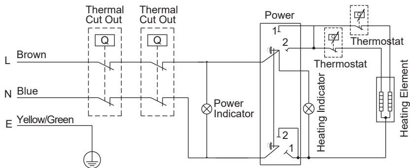
WIRING DIAGRAM
